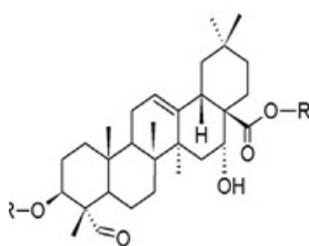
Figure 7: Triterpene glycosides.
