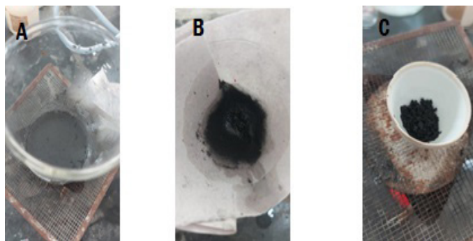
Figure 16: (A) Boiling ash residue (B) Filtration (C) Collection of filtrate
