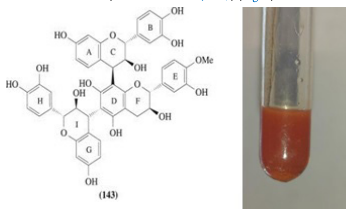
Figure 11: Tetrafucol A.
