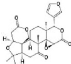
Figure 8: 7,16-Dioxo-7,16-dideoxylimondiol.
