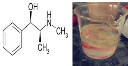
Figure 14: phenethylamine alkaloid.
