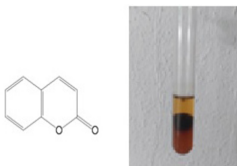
Figure 2: 2H-chromen-2-one.
