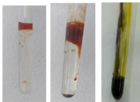
Figure 6: 24-ethyl-lanostane.
